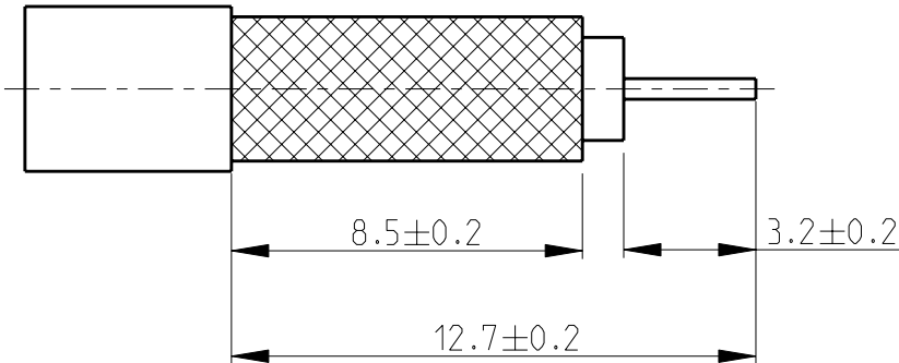
Cable preparation for cable type LMR-240 FR
