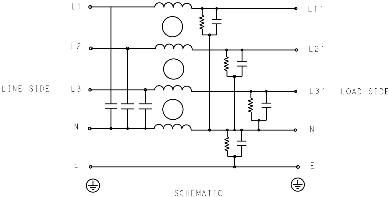
SCHEMATIC
