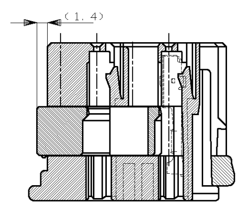
SECT. A-A
