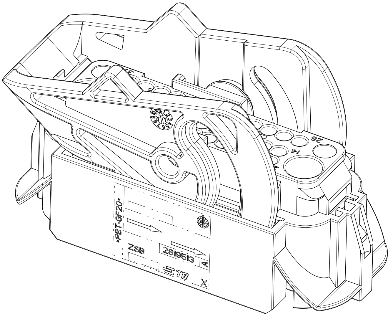
PERSPECTIVE VIEW SCALE 2:1
