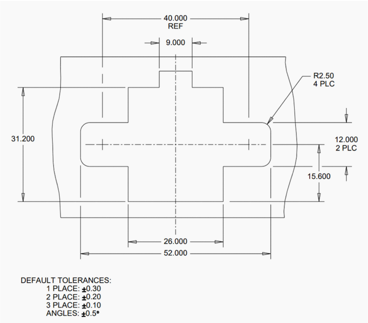
PANEL CUTOUT VIEW
