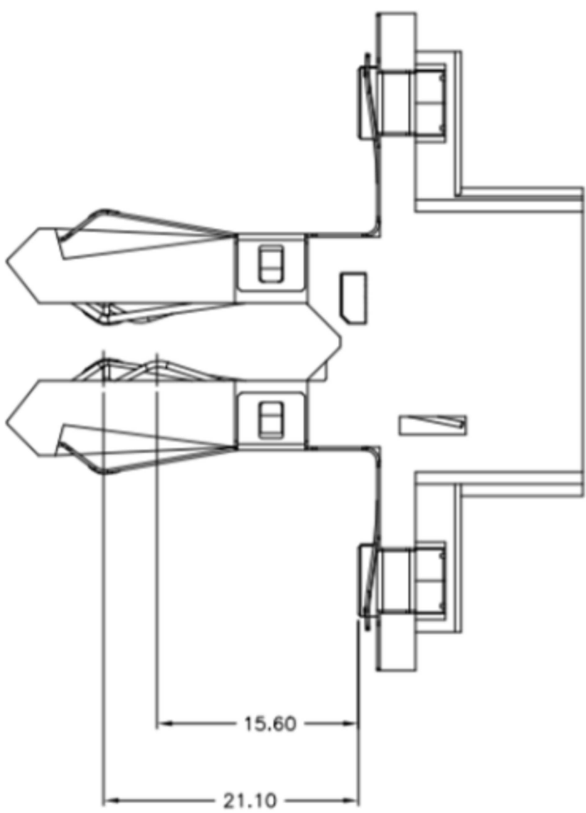
PLANE SIDE
