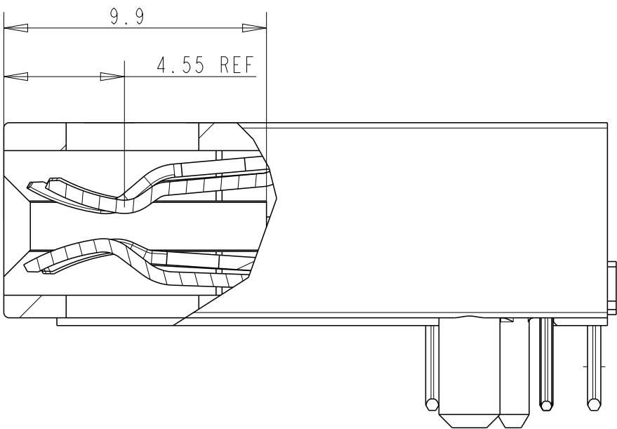
SECTION P-P
