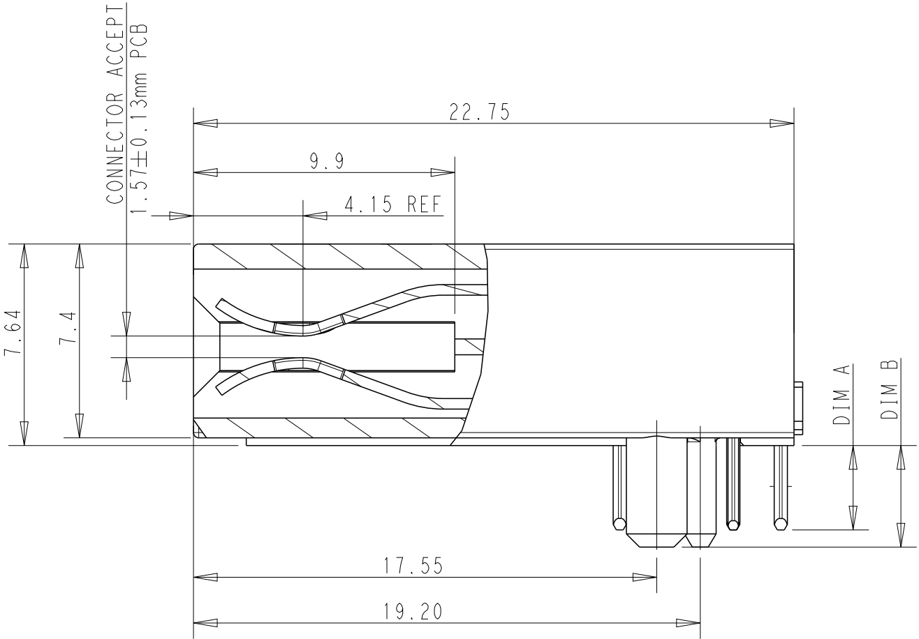
SECTION S-S
