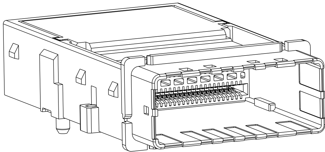
2373624-5 AND 1-2373624-1 AS SHOWN UNSPECIFIED DIMENSIONS ARE SAME AS 2373624-4 SCALE 3:1
