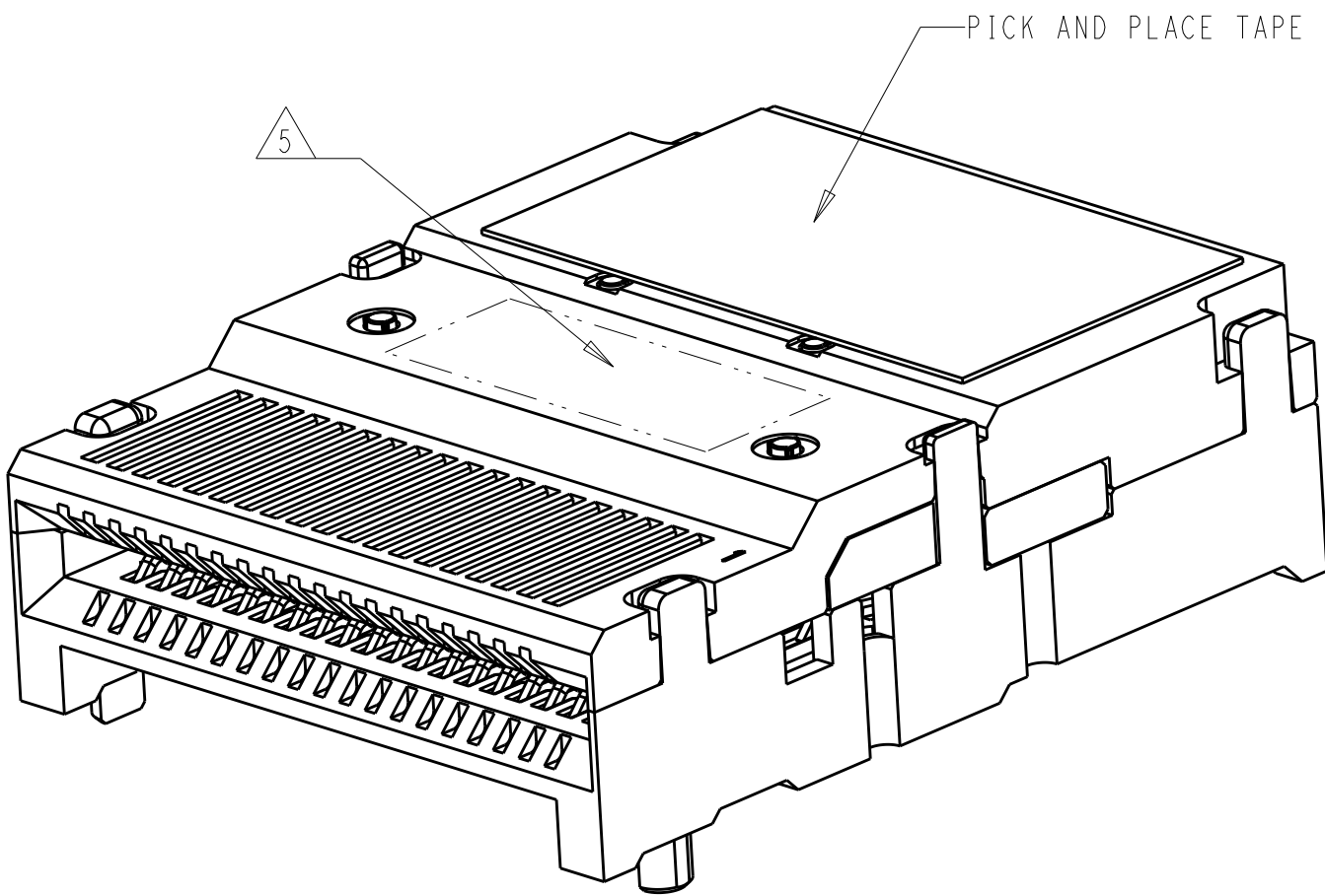
2360945-3 ISO VIEW AS SHOWN SCALE 6:1
