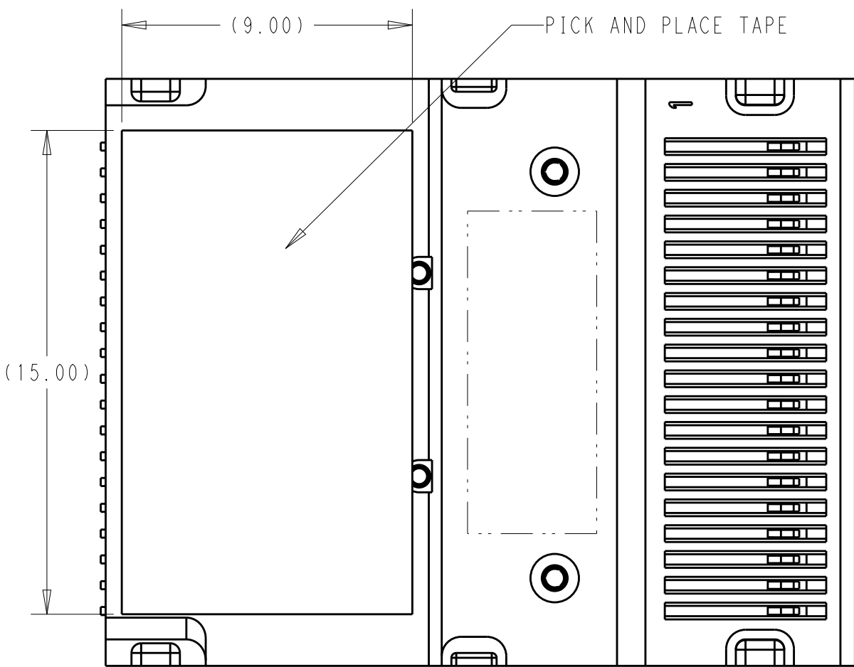
2360945-3 AS SHOWN SCALE 6:1
