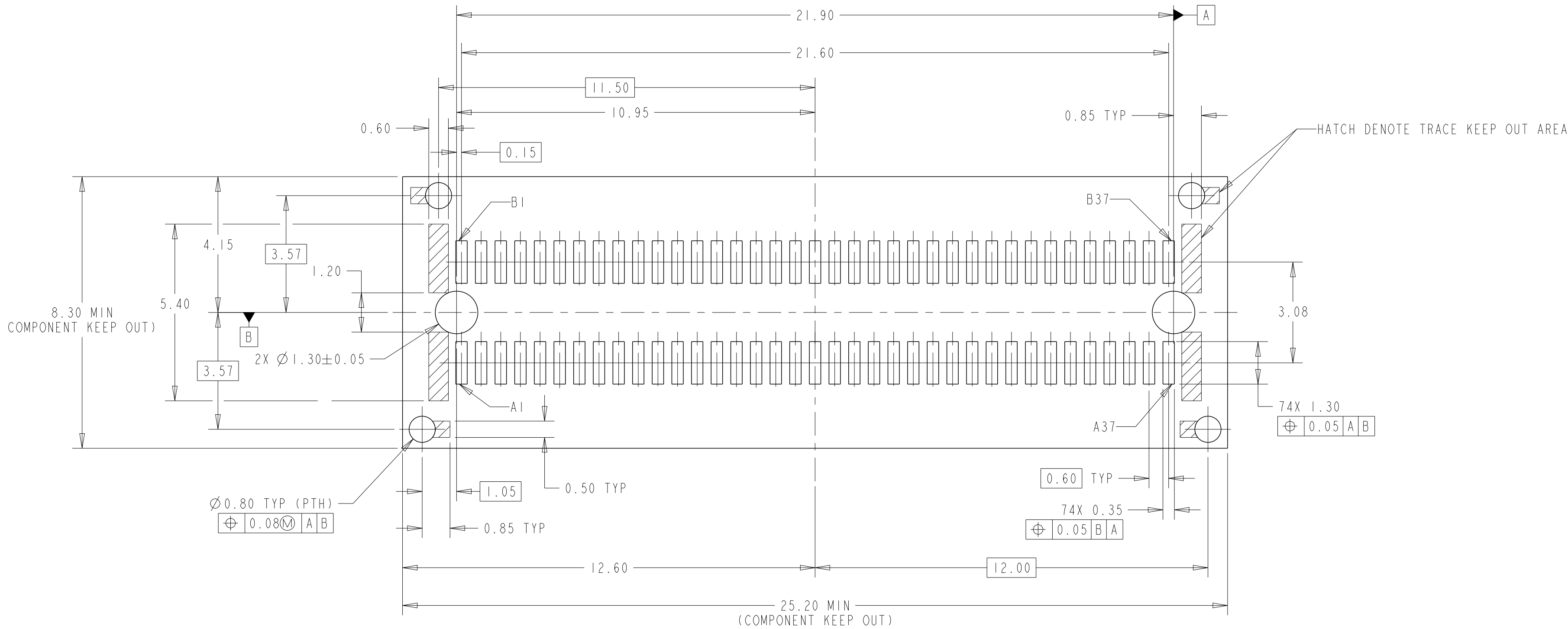
RECOMMENDED PCB LAYOUT AND KEEP OUT AREA SCALE 10:1
