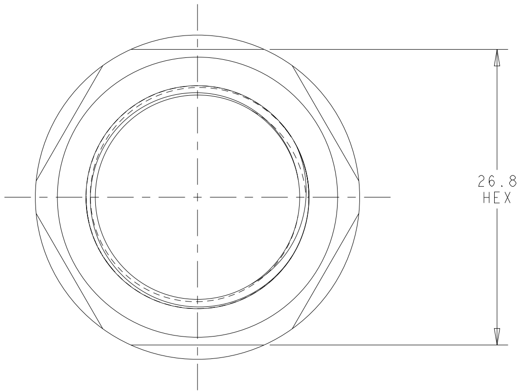
LOCKING NUT DETAIL SCALE: 3:1
