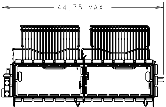
2337452-3 AS SHOWN W/ 2LEFT LIGHT PIPE SCALE 2:1
