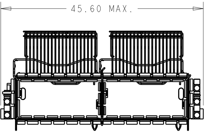
2337452-1 W/ 2LEFT+ 3RIGHT LIGHT PIPE SCALE 2:1
