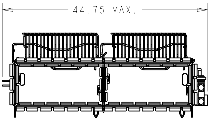
2337452-4 AS SHOWN W/ 2RIGHT LIGHT PIPE SCALE 2:1
