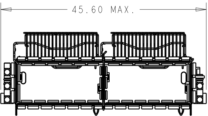
2337452-2 AS SHOWN W/ 3LEFT+ 2RIGHT LIGHT PIPE SCALE 2:1
