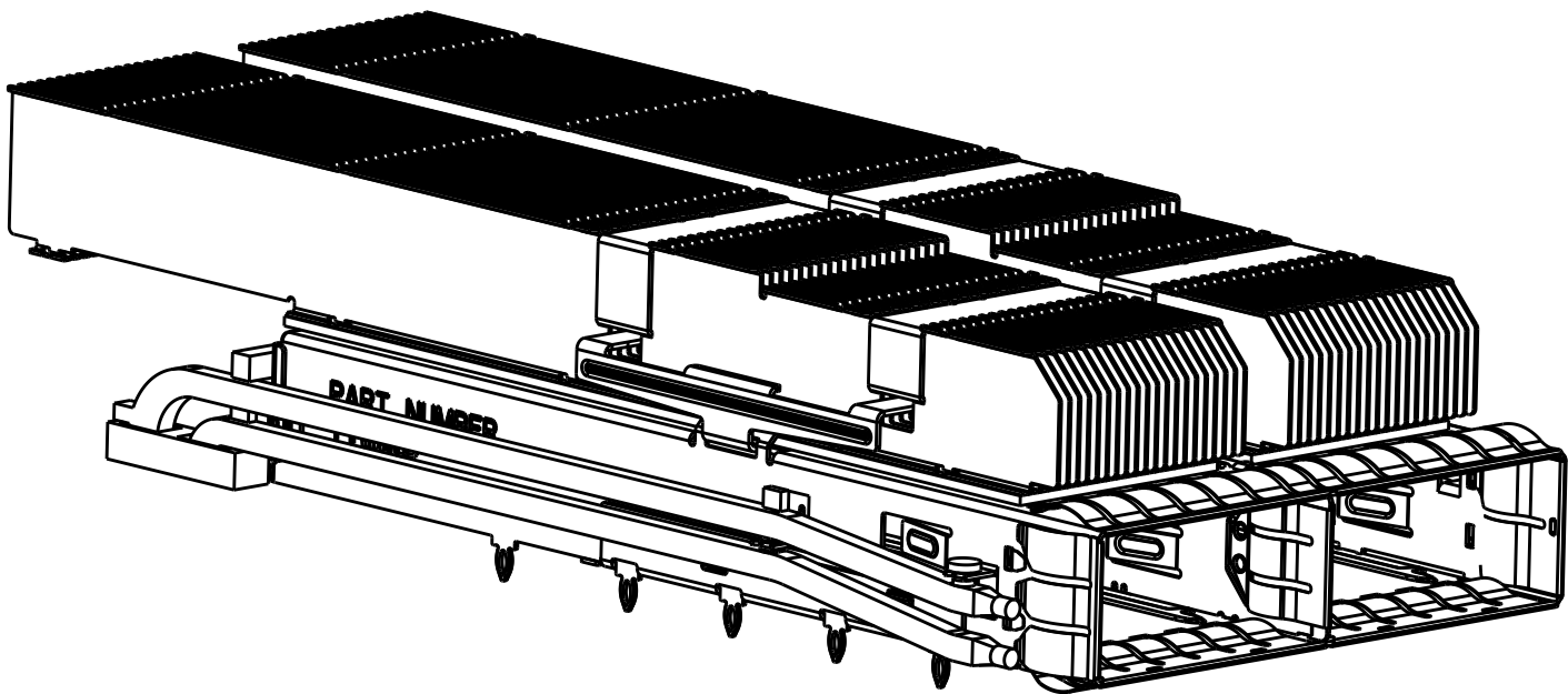
2337452-1 AS SHOWN SCALE 2:1
