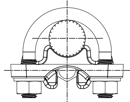
Cable 11/16 to 15/16 assembly
