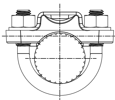
Cable 15/16 to 1 11/16 assembly
