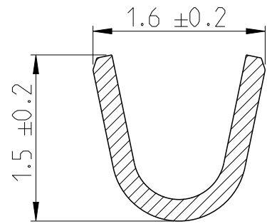
SECTION K-K 20:1
