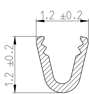
SECTION J-J 20:1
