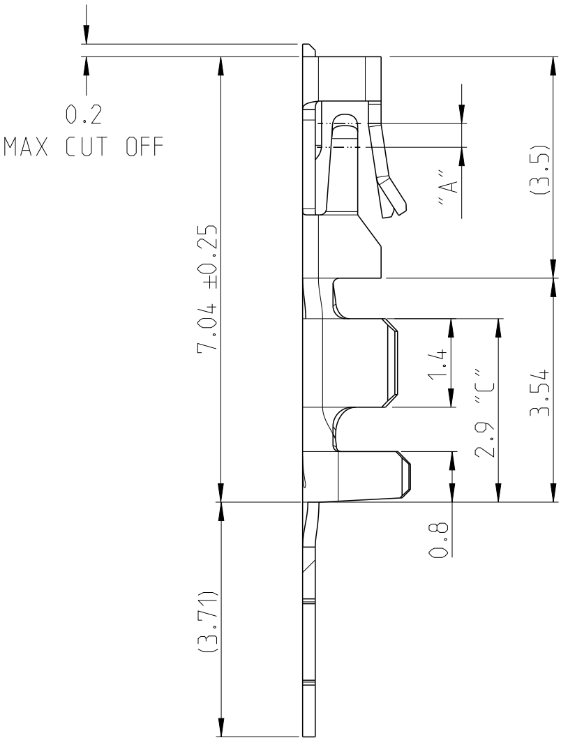
SECTION U-U
