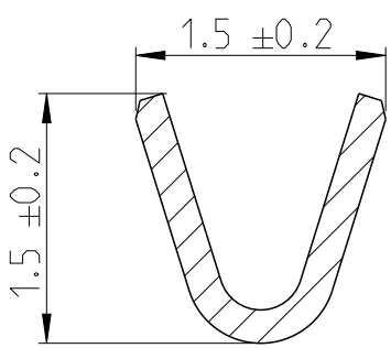
SECTION J-J 20:1
