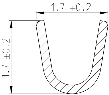
SECTION K-K 20:1
