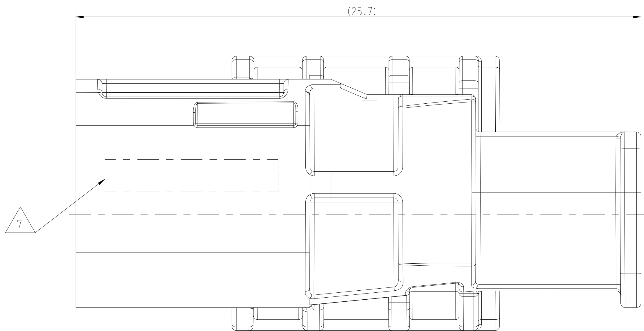
SECTION B-B
