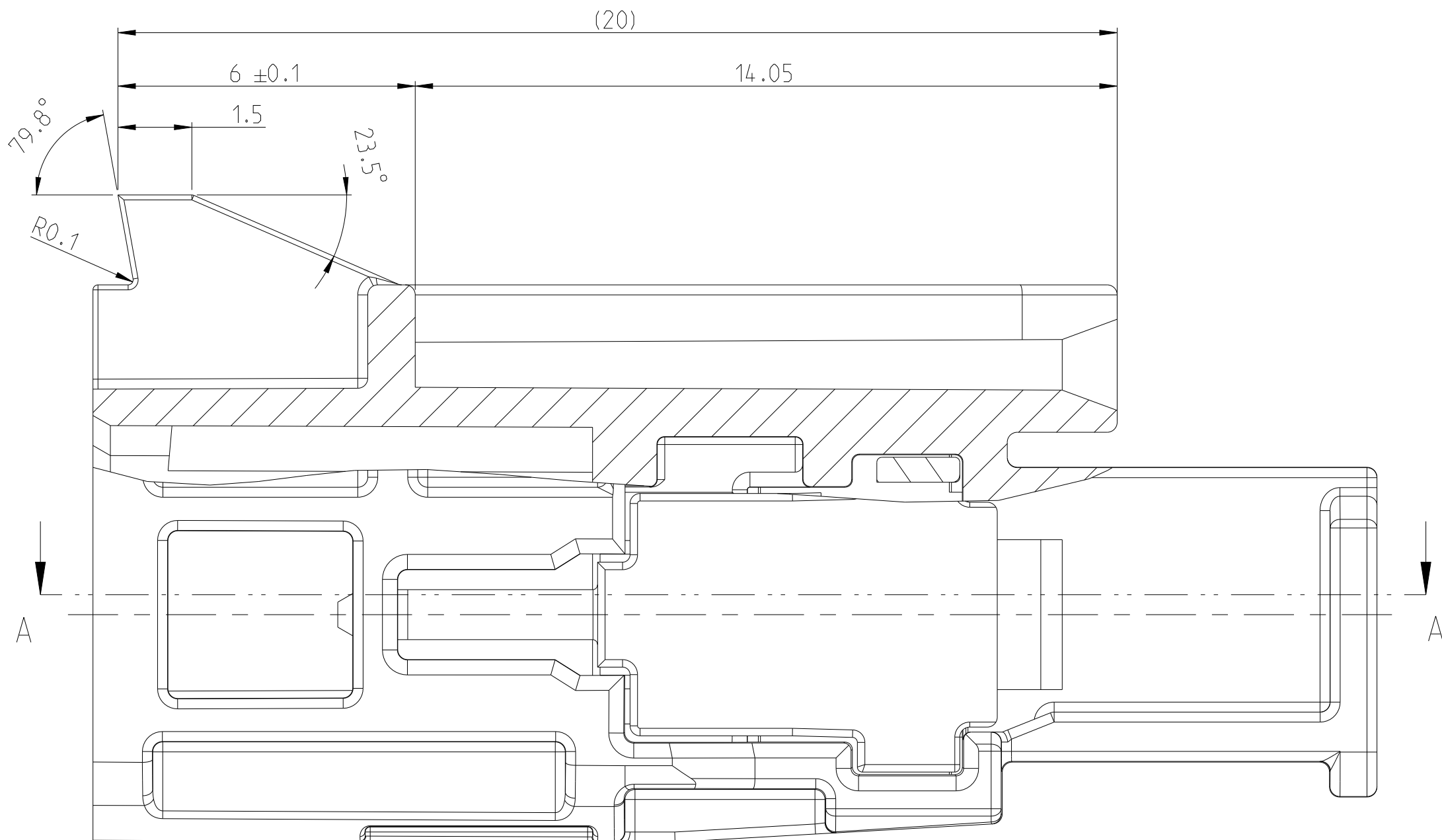
SECTION B-B
