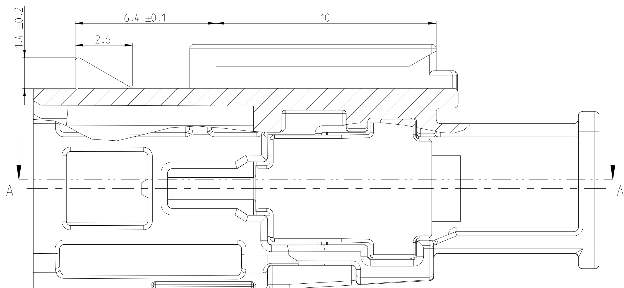
SECTION B-B
