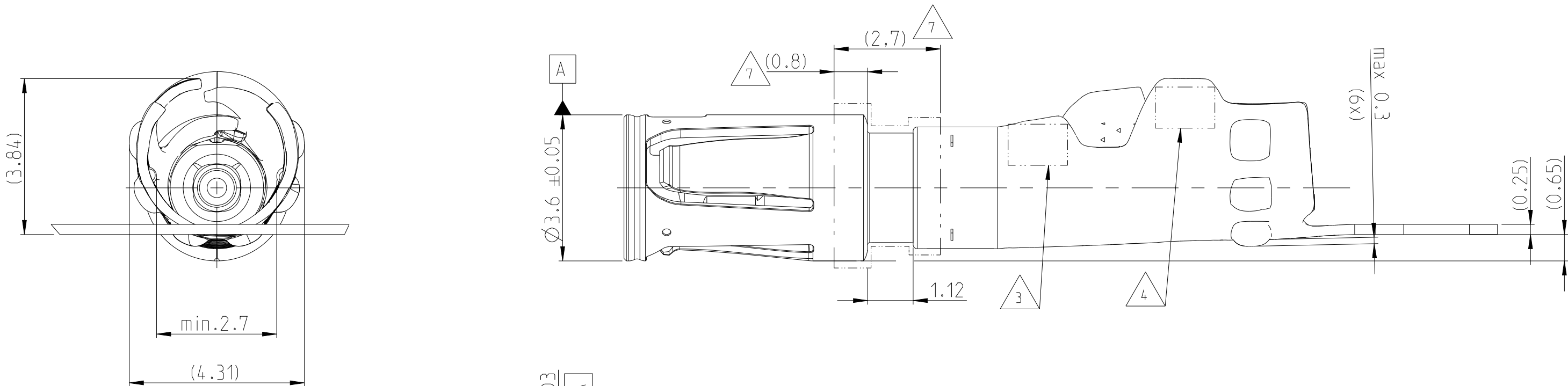
SECTION Q-Q
