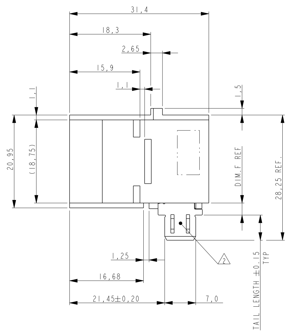
THE CONFIGURATION WITHOUT DIMPLES PRODUCT NUMBER 2178531-2/-4/-7
