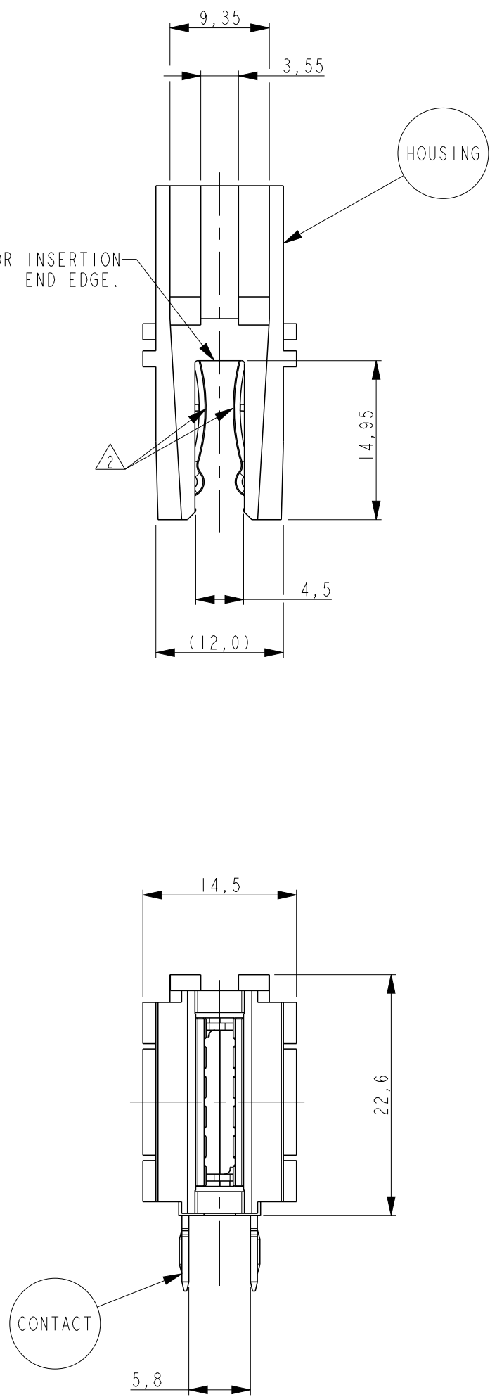
THE CONFIGURATION WITH DIMPLES PRODUCT NUMBER 2178531-1/-3
