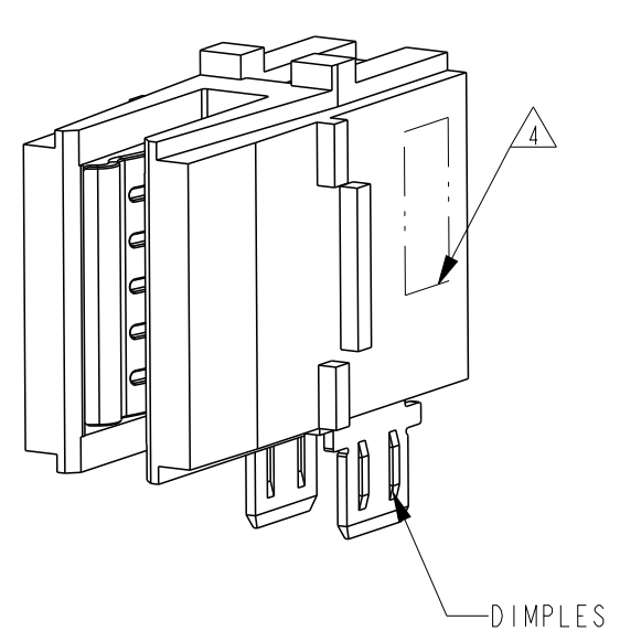
THE CONFIGURATION WITH DIMPLES PRODUCT NUMBER 2178531-1/-3
