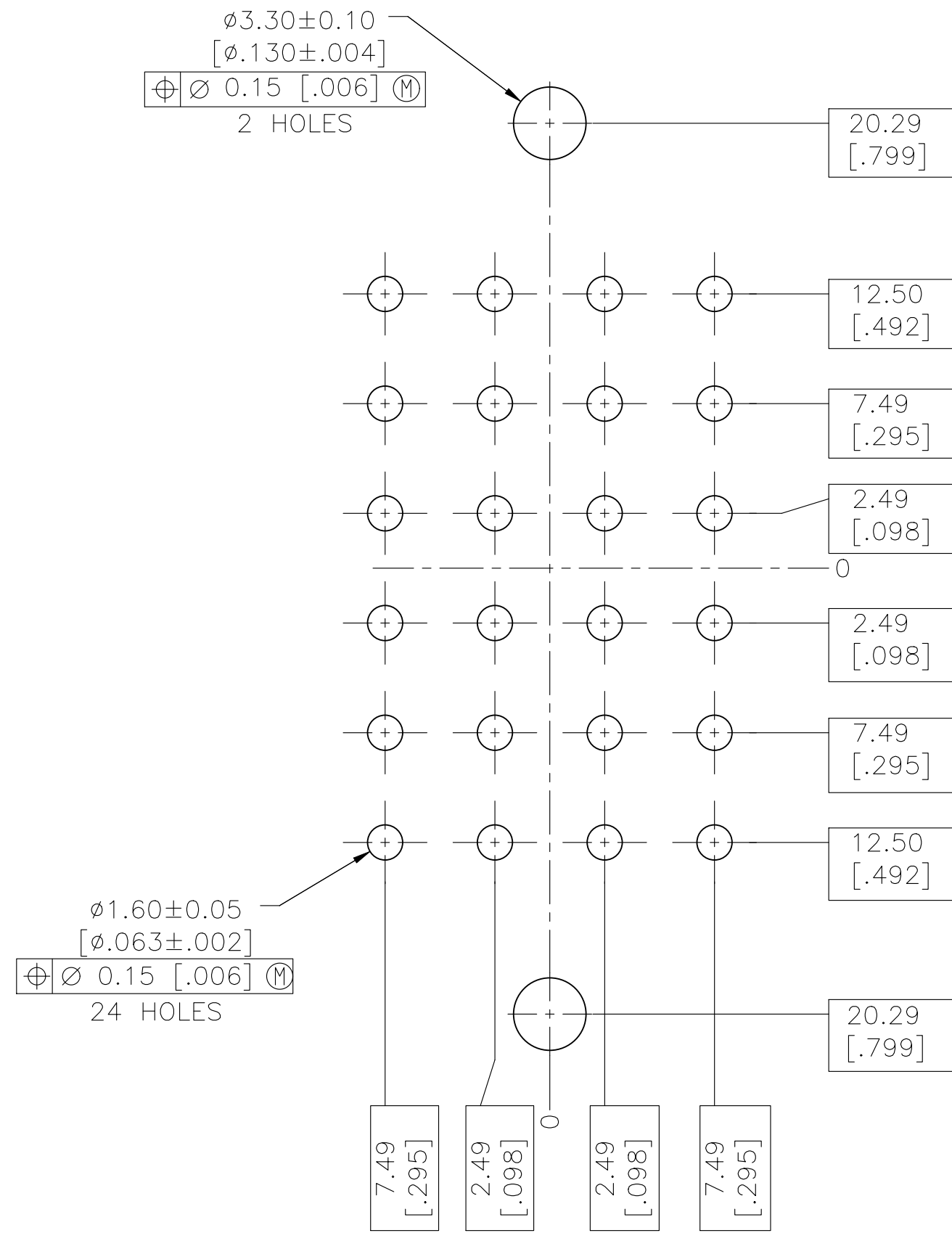
RECOMMENDED LAYOUT
