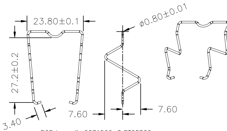
PCB type clip 2071566-8 PT28P00
