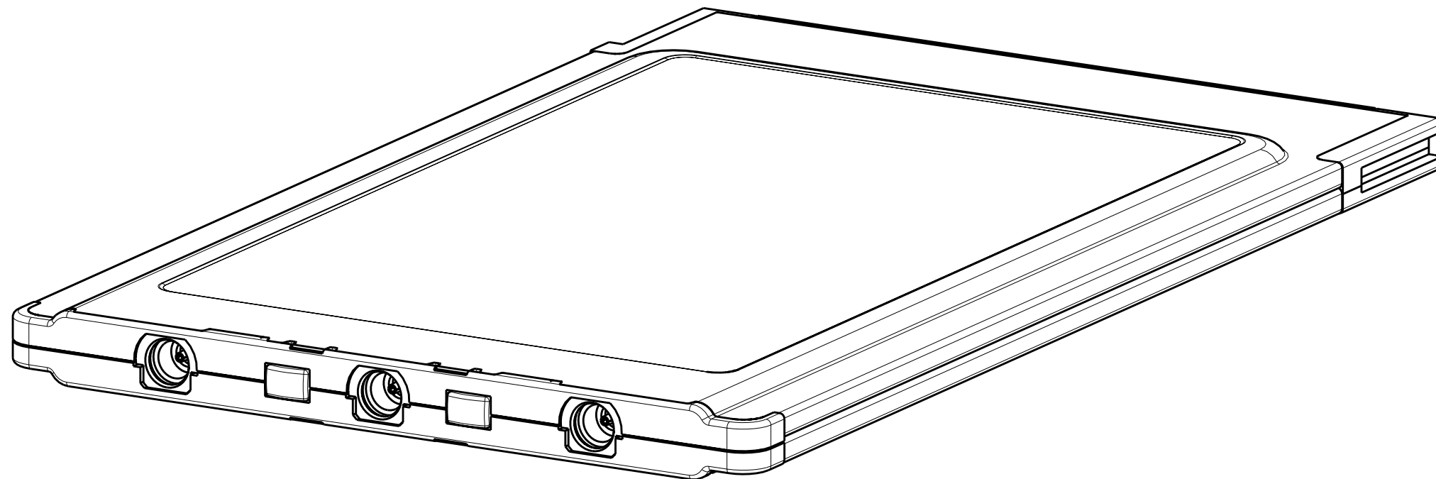
FULLY ASSEMBLED CARD 3X MMCX JACK END SCALE 3:1
