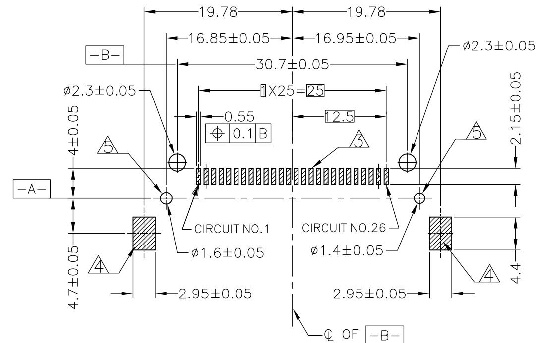
RECOMMENDED PCB LAYOUT (TOLERANCE ±0.05)
