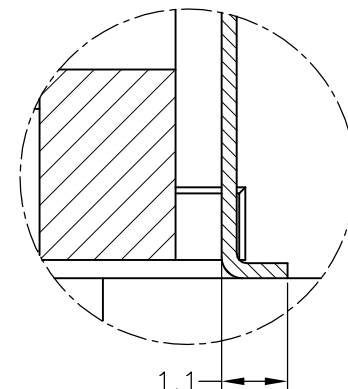
DETAIL E (SCALE 8:1)
