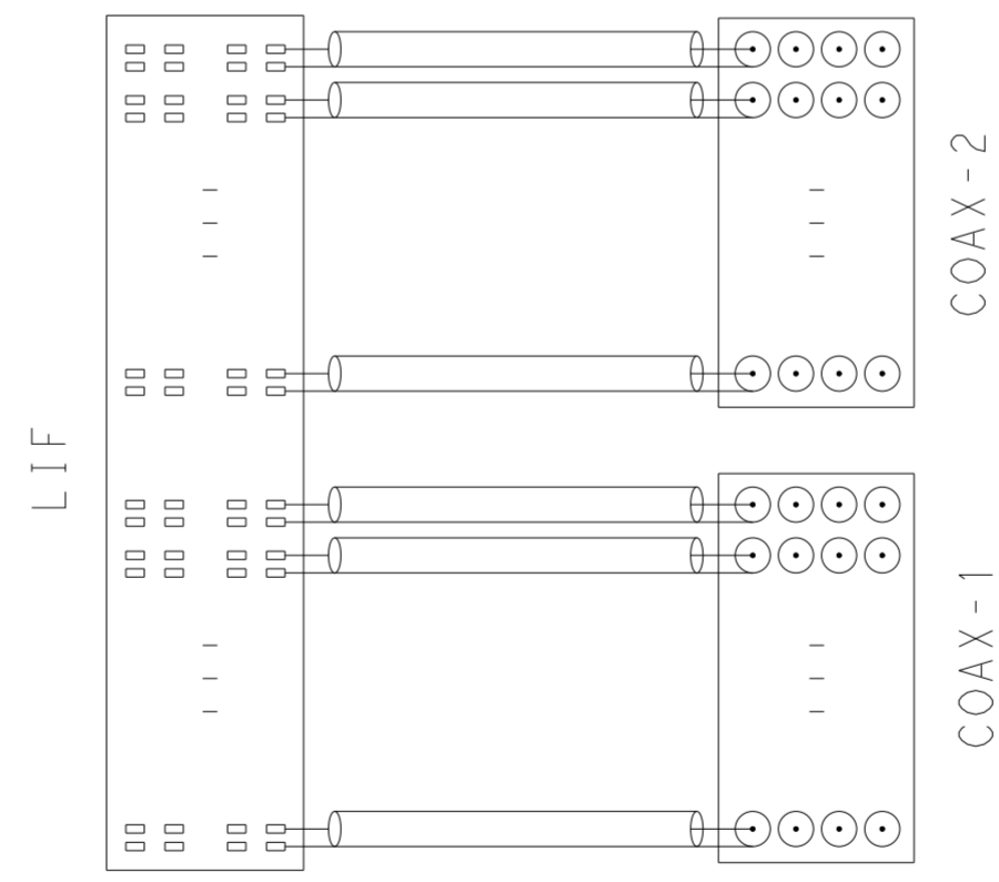
4 WIRING DIAGRAM
