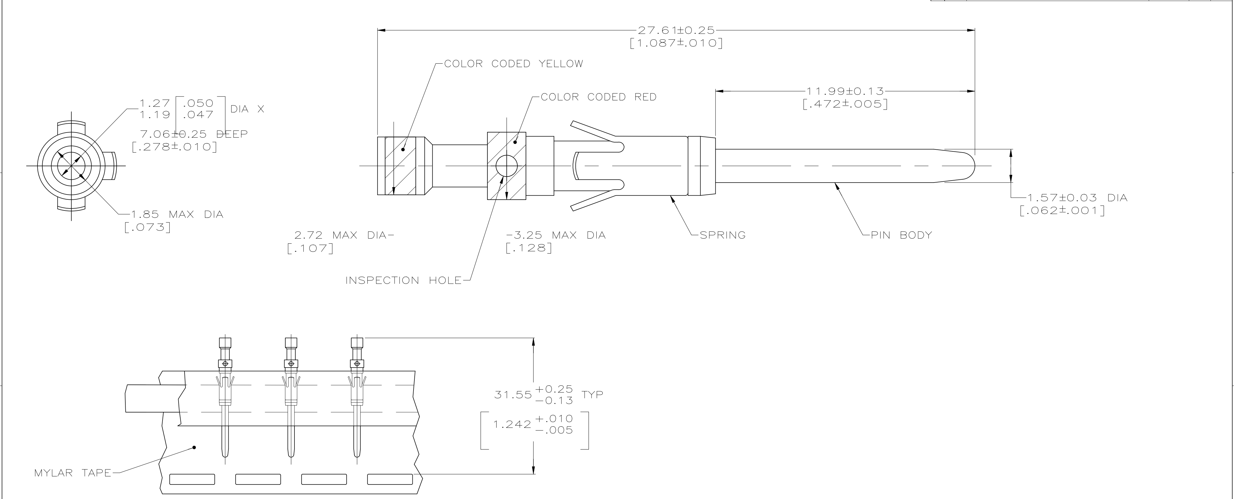
TAPE MTG DETAIL SCALE 2:1
