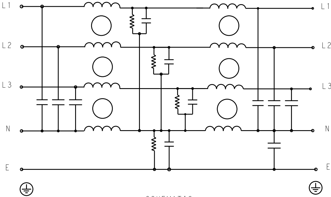
SCHEMATIC
