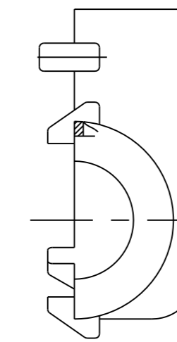
SECTION C-C SCALE 2:1
