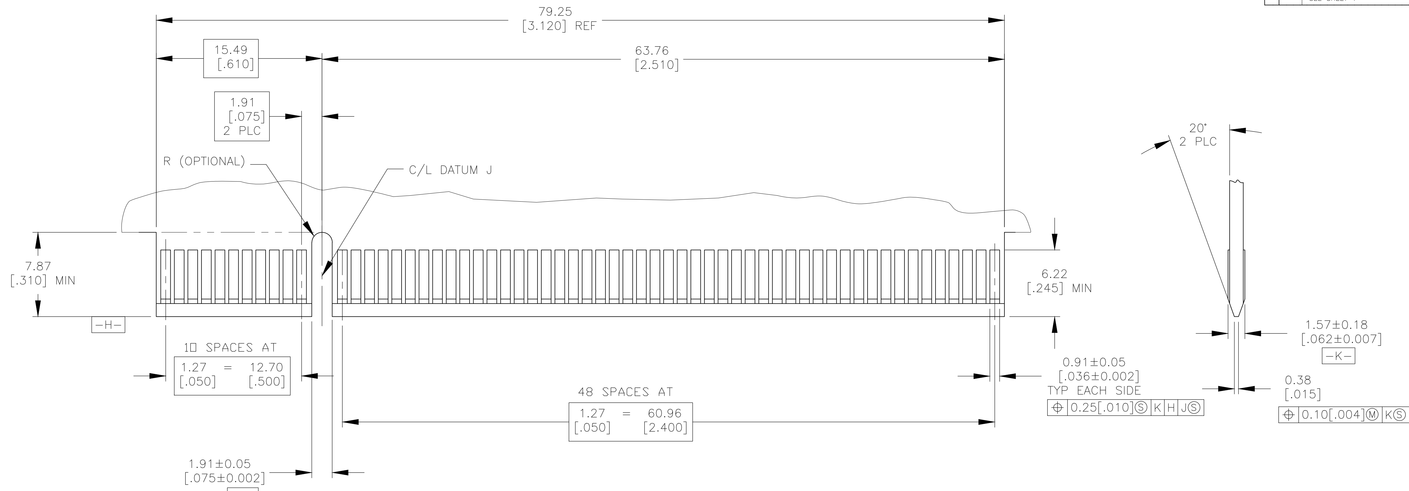
RECOMMENDED MATING BOARD EDGE CONFIGURATION
