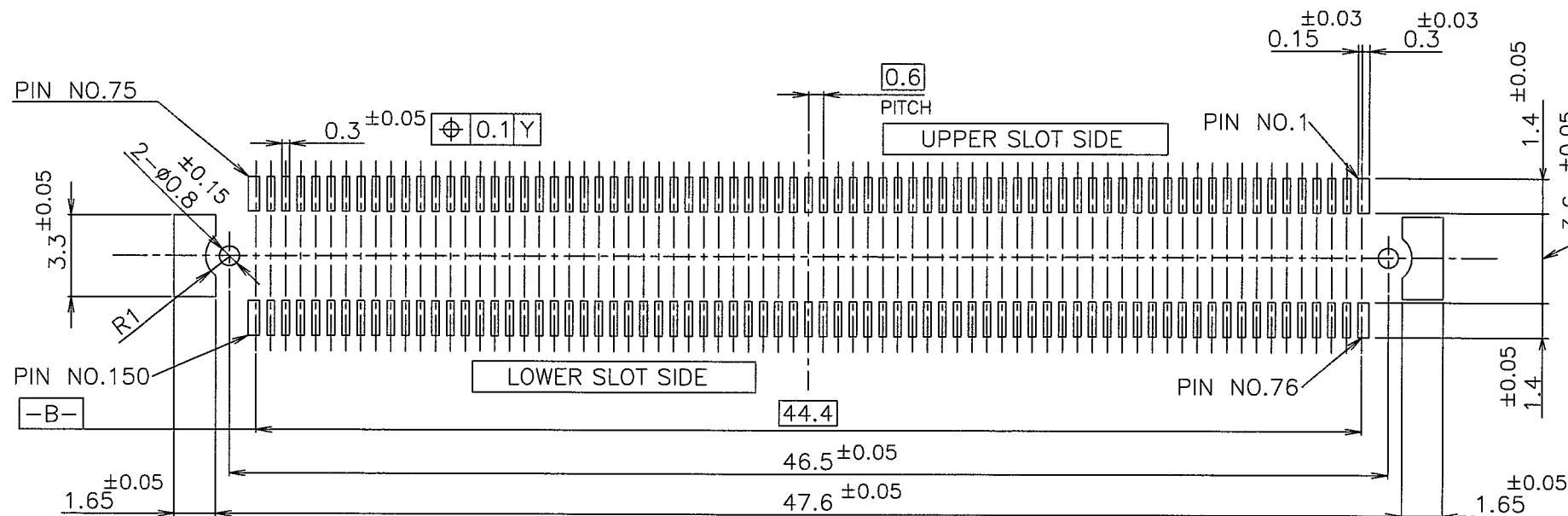
DETAIL H
