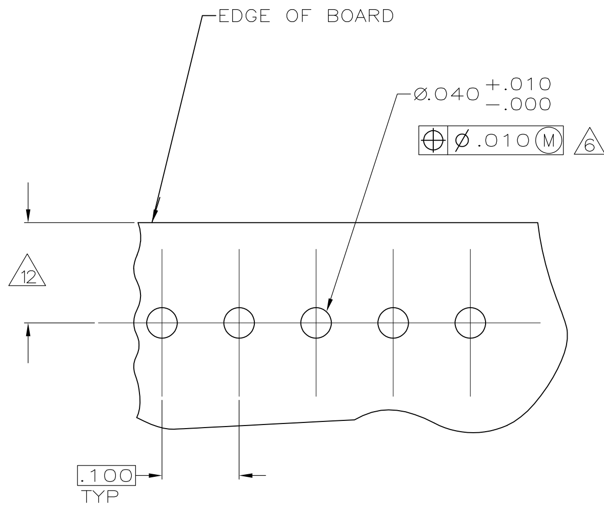
RECOMMENDED MOUNTING HOLE PATTERN FOR .063 THICK P.C. BOARD
