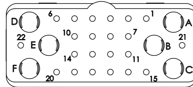
MATING FACE
