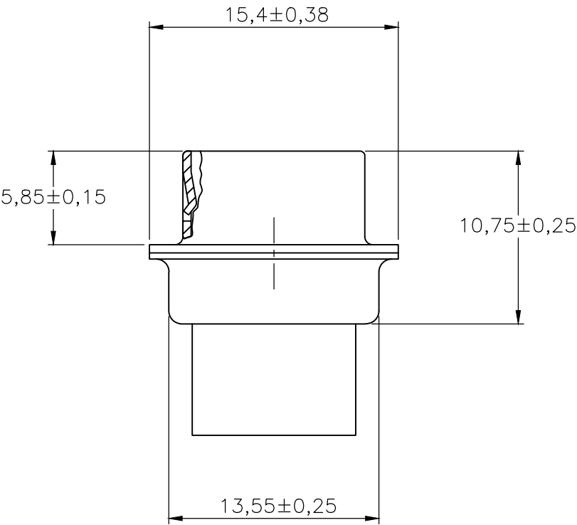
SIZE 5 CONFIGURATION
