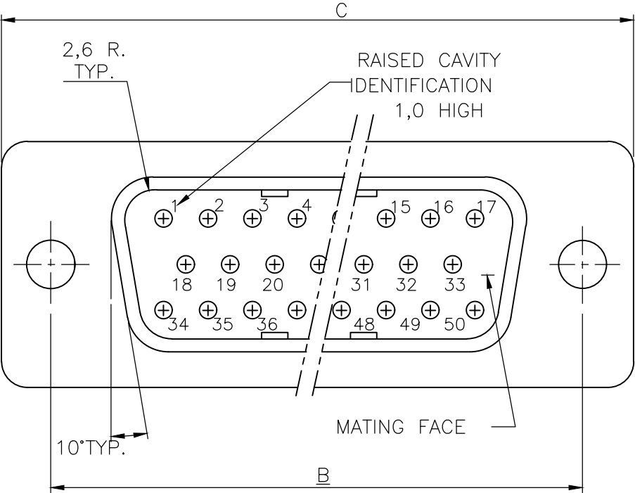
SIZE 5 CONFIGURATION
