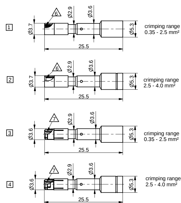
power contact type: 2 mm scale 2 : 1
