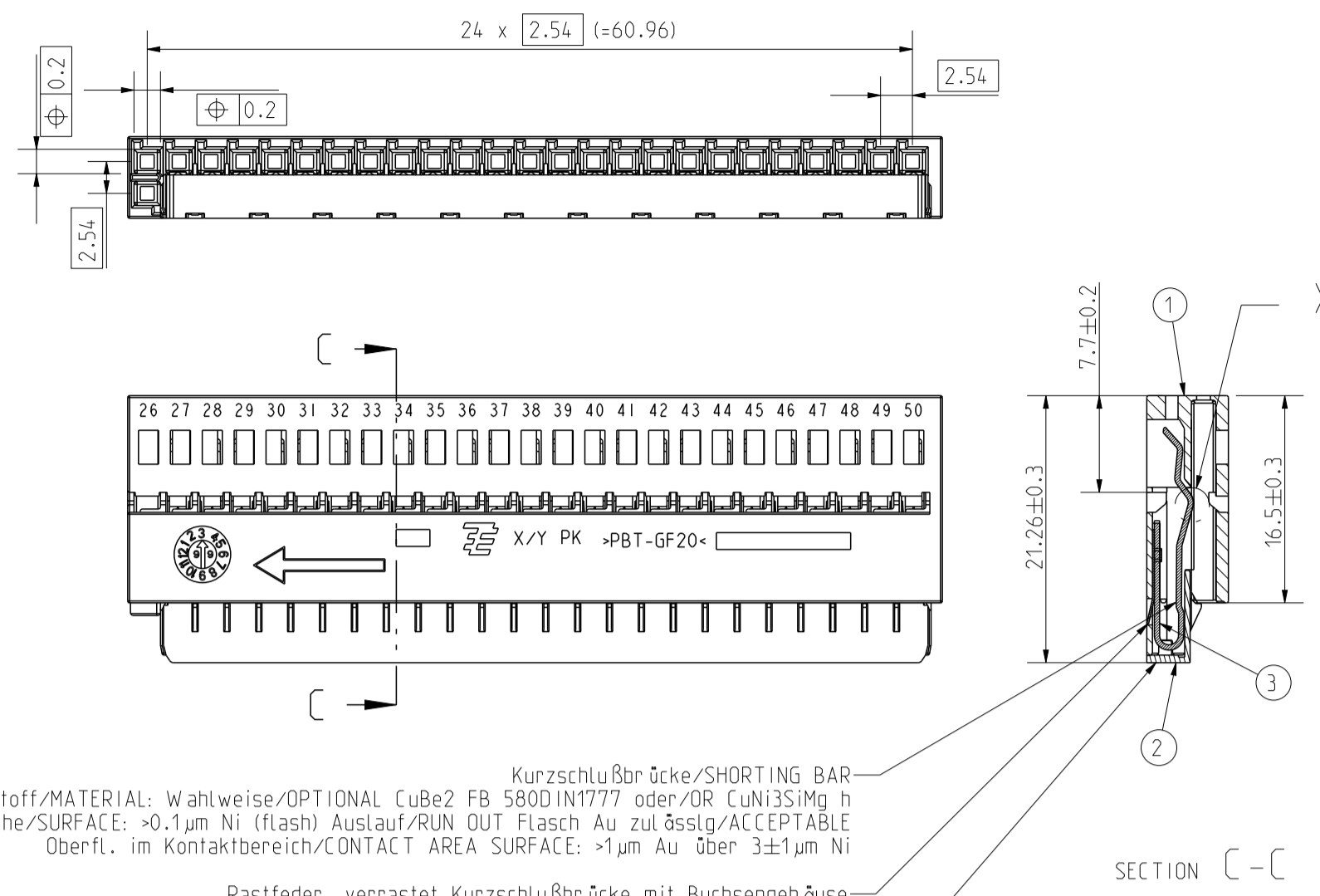
SECTION C-C
