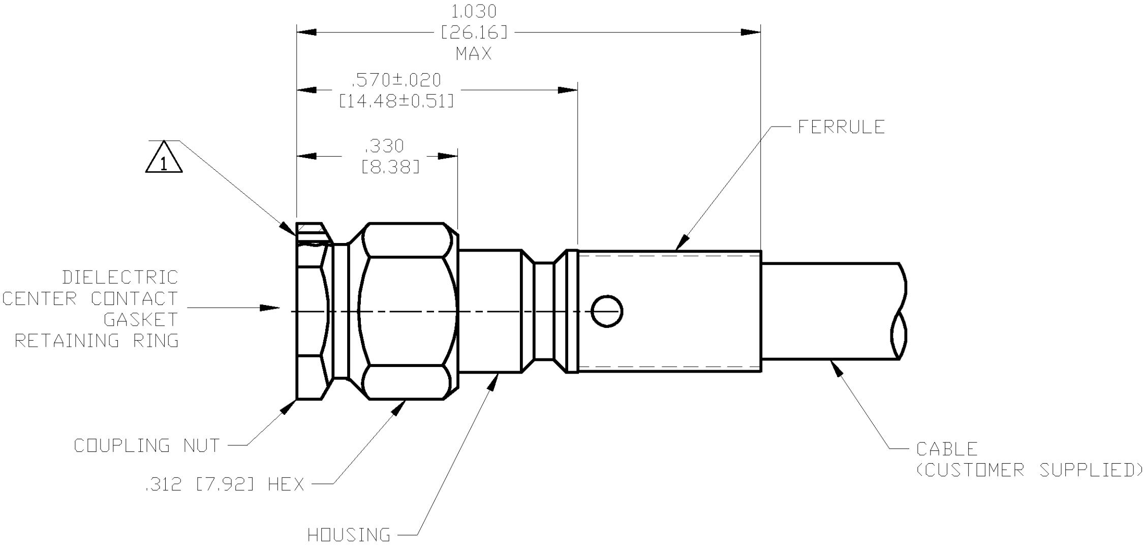
ASSEMBLED VIEW
