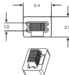
Part No. 1-1442004-7
