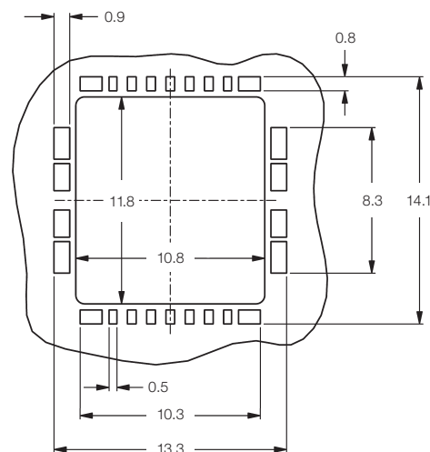
PCB Layout
