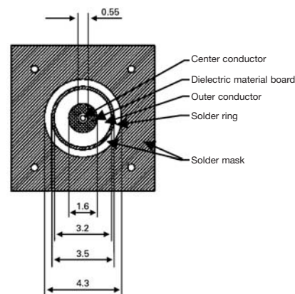
PCB Pattern
