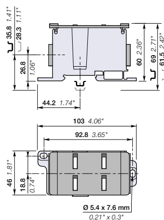
46 mm 1.81 in spacing
