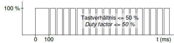
Spulenerregung [V] / Coil energizing [V]
