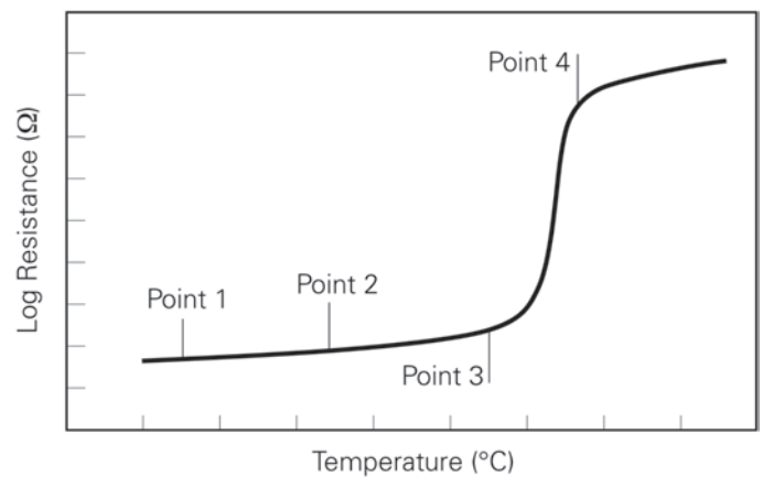
Figure 2 - Example of Operating Curve for PPTC Devices.
