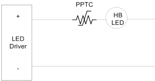
Figure 1 - Typical PPTC circuit protection design for HB LEDs.
