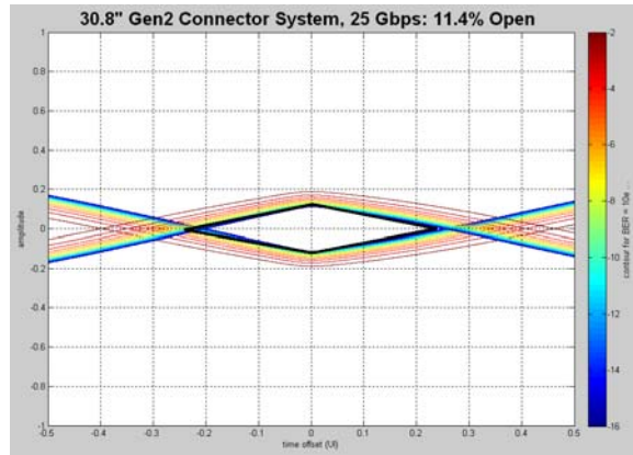
Figure A6a: 30.8" Gen2, 100 Ohm System Performance – Throughput Only
