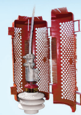
BUSHING & ARRESTER COVERS
