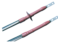
HEAT SHRINK TERMINATIONS UP TO 123 kV
