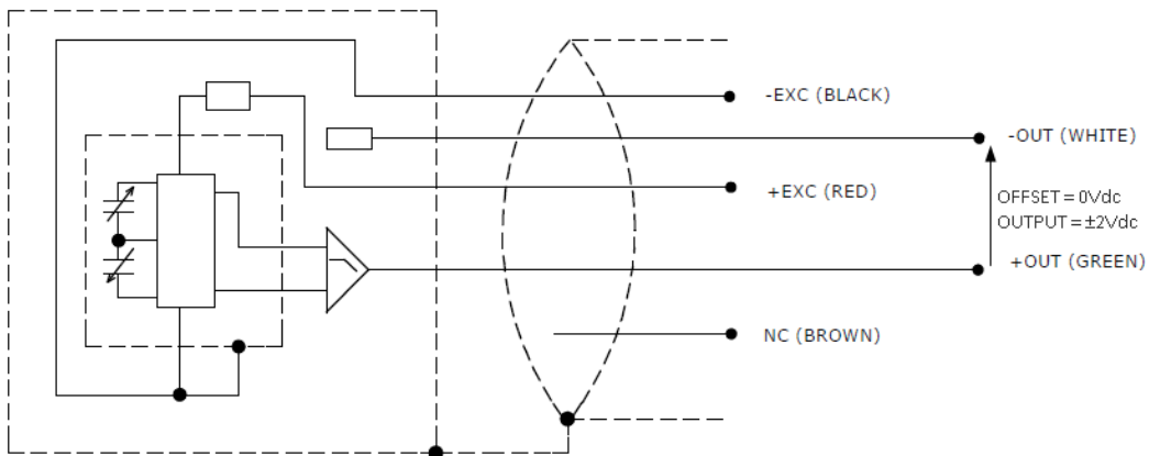
DIFFERENTIAL OUTPUT
