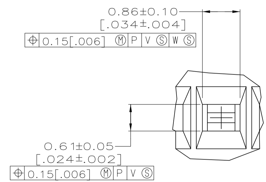
DETAIL T SCALE 20:1 TYPICAL
