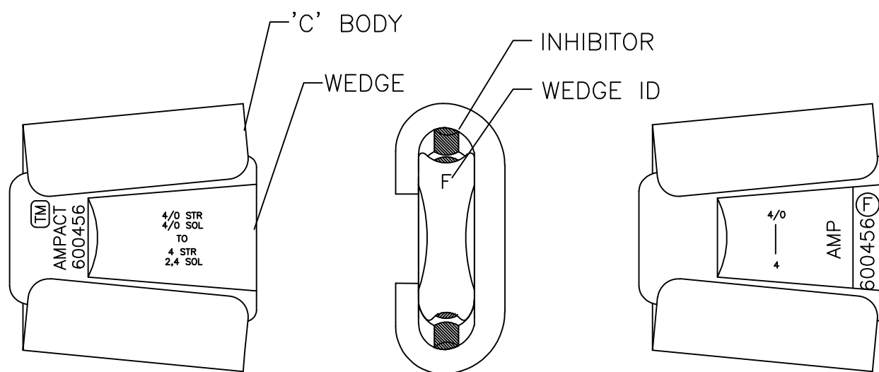
ALTERNATE MARKING ON WEDGE
