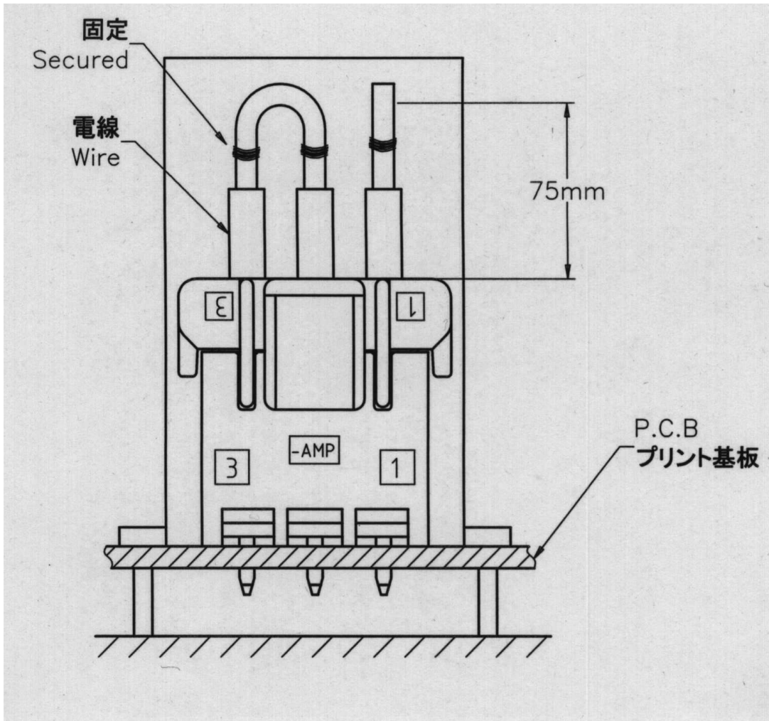
Fig. 6 低周波振動、物理的衝撃のコネクタ取付方法 Fig. 6 Connector Mounting Methods of Low Frequency Vibration and Physical Shock Tests
