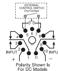
Wiring Diagrams (Bottom Views)
