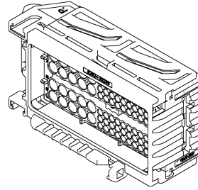
74Pos Plug Housing Assembly THS STD Type
