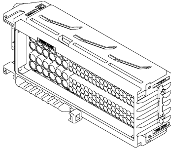
89/126Pos Plug Housing Assembly STD Type
