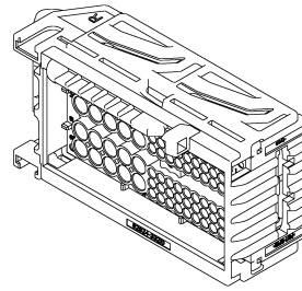
74Pos Plug Housing Assembly THS Reverse Type
