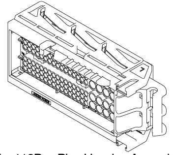
112Pos Plug Housing Assembly THS Reverse Type
