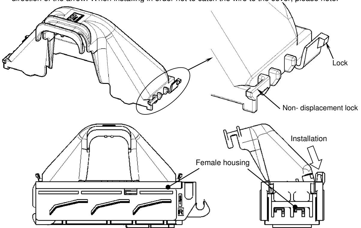
126Pos Wire Cover Fig.21
