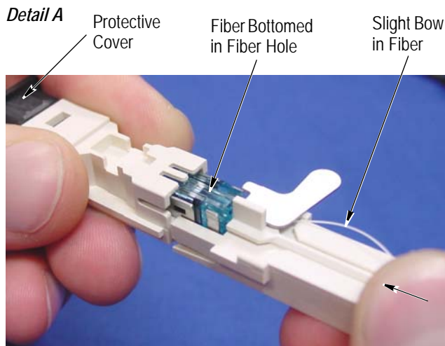
Insert Fiber into Fiber Hole
