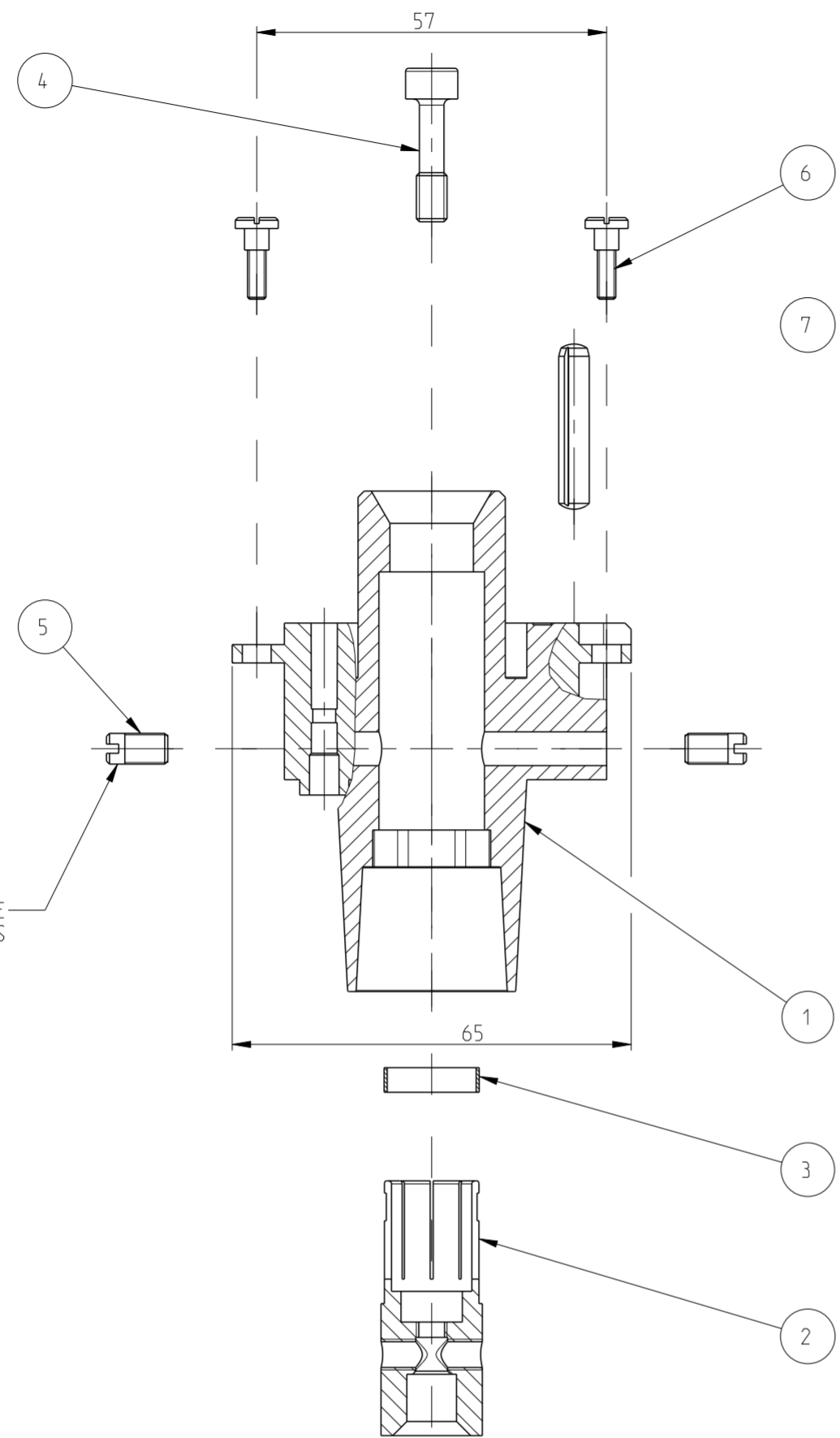
SCREW VARIANT
