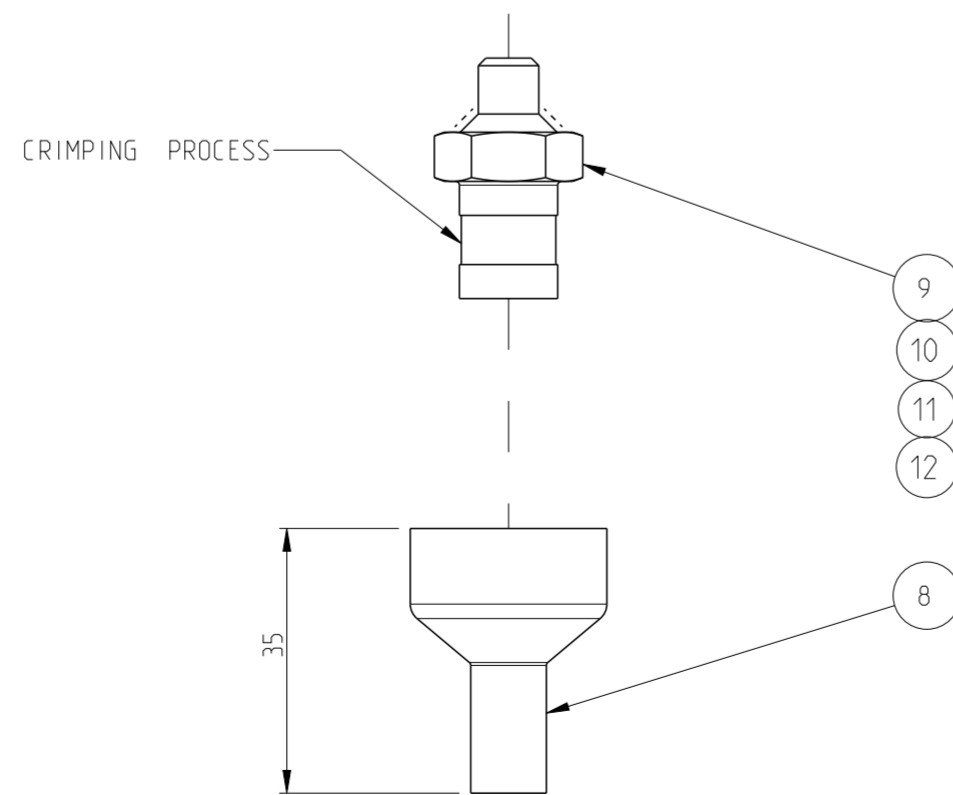
SCREW VARIANT
