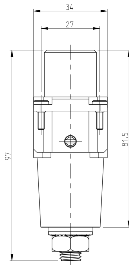
PIN/BOLTING TERMINATION VARIANT
