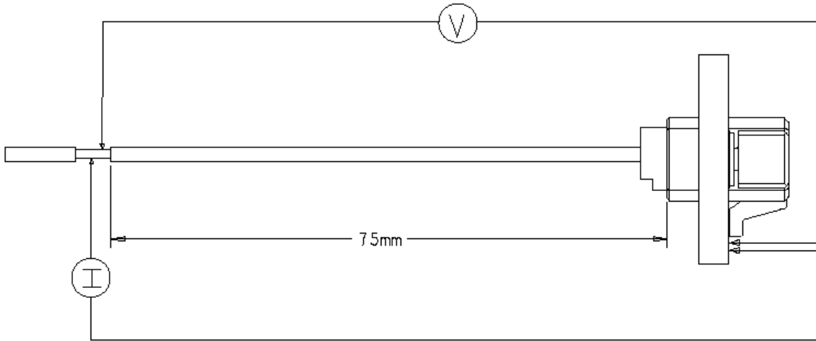
Figure 3 LLCR Measurement Points
