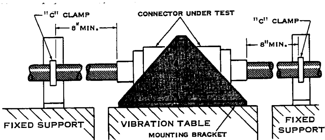
Figure 4 Vibration & Physical Shock Mounting Fixture
